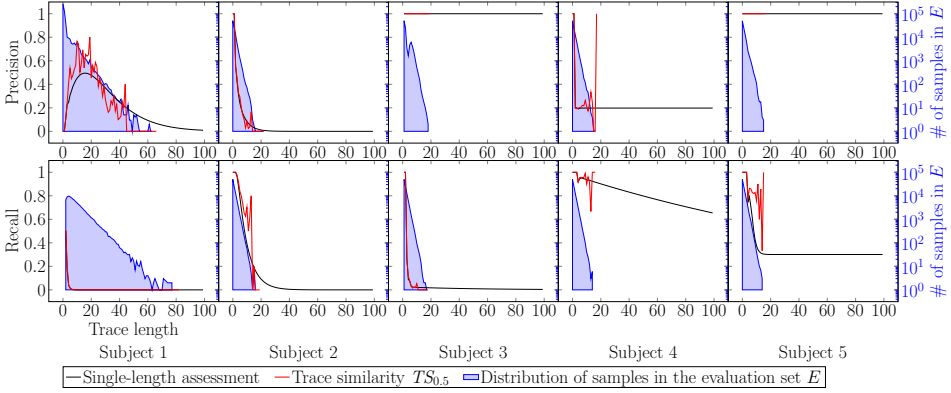
(a) Trace similarity using a random walk with p_a = 0.5
