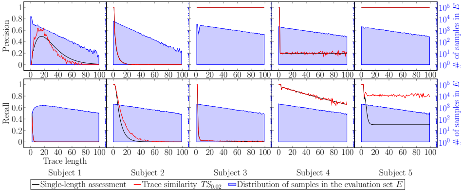
(c) Trace similarity using a random walk with p_a = 0.02
