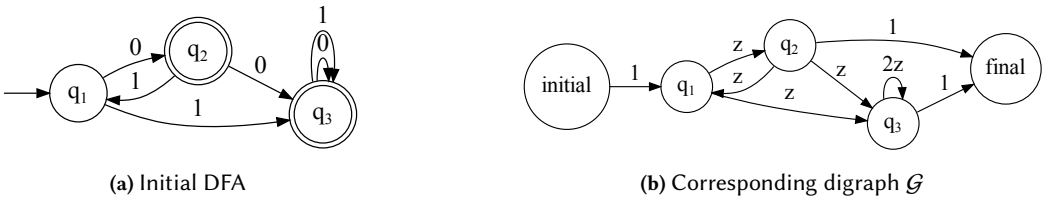
Fig. 4. Example of digraph construction
