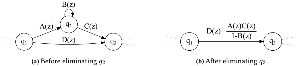
Fig. 5. Node elimination
