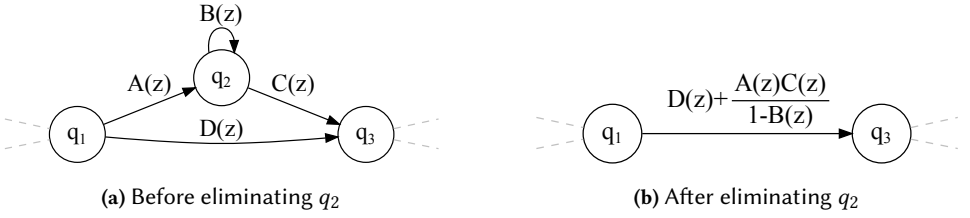
Fig. 5. Node elimination
