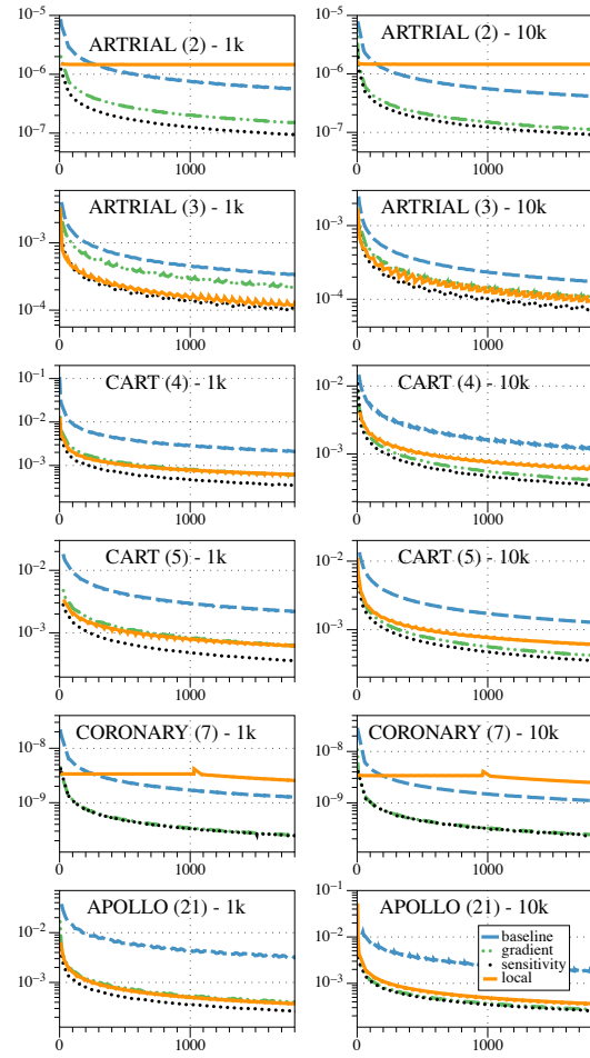
Figure 2: Convergence rate of iterative sampling and the baseline approach on selected subjects (y-axis in logarithmic scale).
