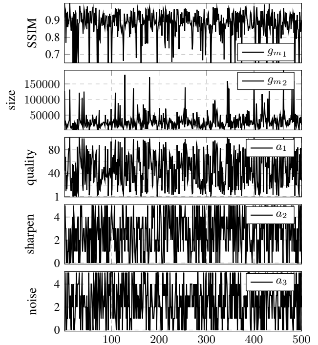
Fig. 1: Results for the video experiment with the Obama Victory Speech video, with the random adaptation strategy.
