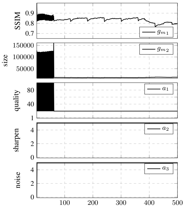
Fig. 2: Results for the video experiment with the Obama Victory Speech video, with the bangbang adaptation strategy and a setpoint of 0.7 for the SSIM and 10000 for the size.
