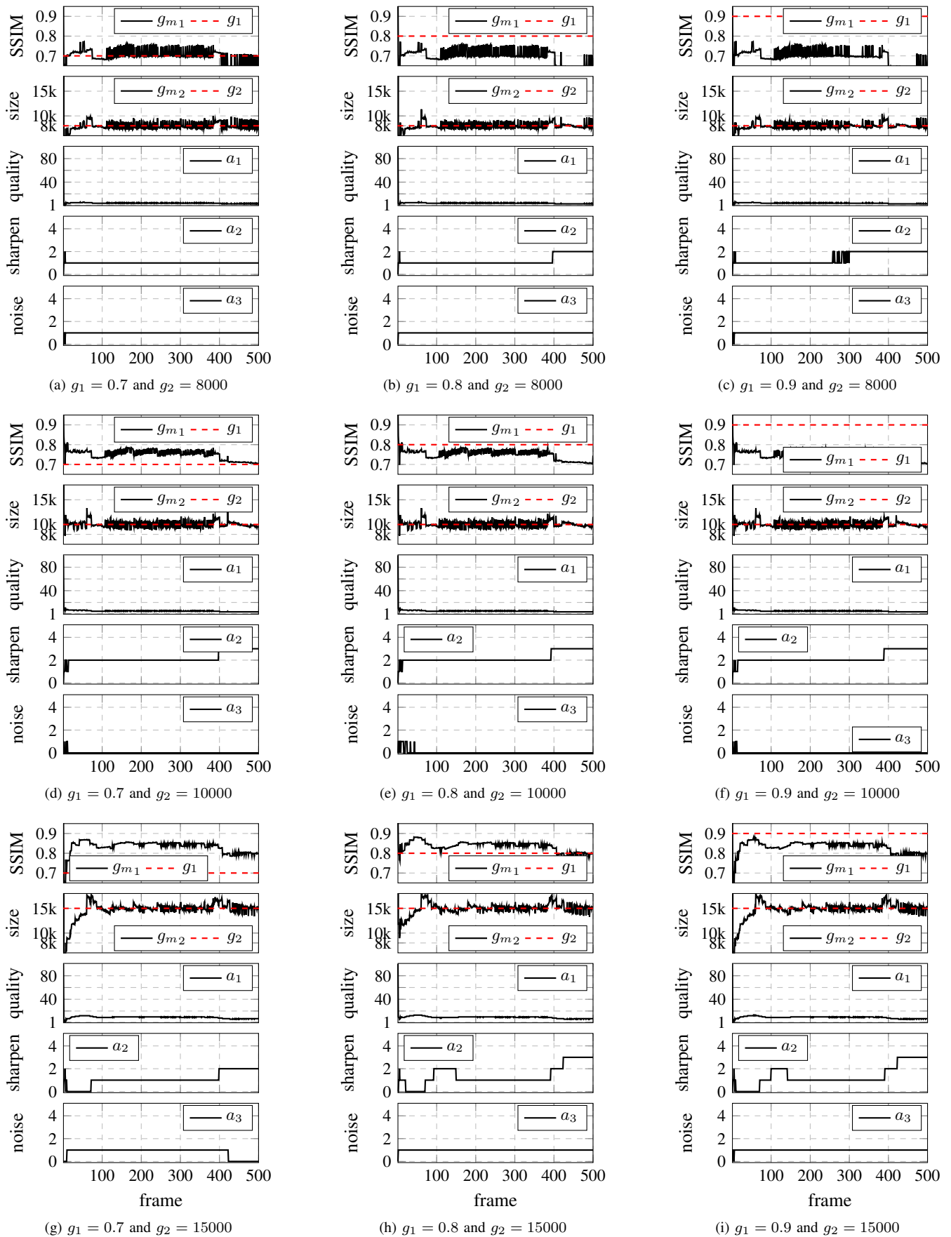
Fig. 3: Results for the video experiment with the Obama Victory Speech video, with the mpc controller, various setpoints for both the size and the SSIM.
