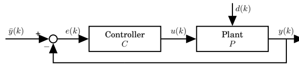
Fig. 2. Adaptive system: the control perspective . This figure originally appeared in [Fileri et al. 2015b].
